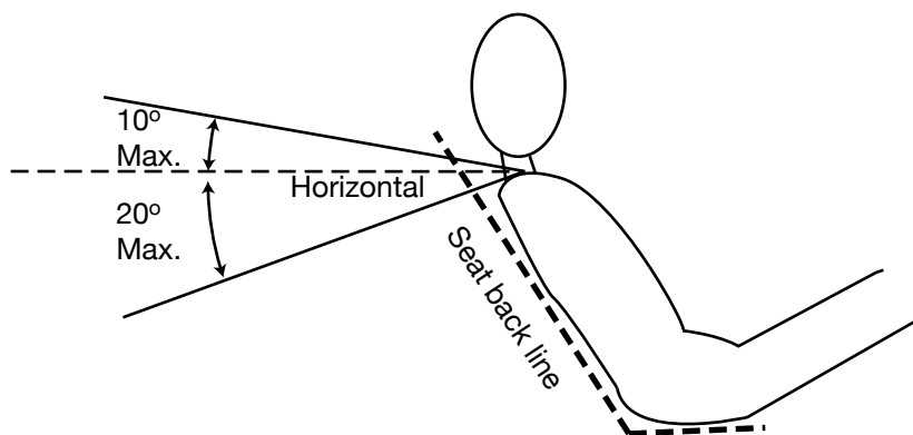
FIGURE 12 Shoulder Harness Angle
